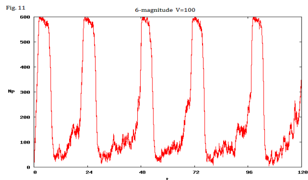
Figure 11: 6-magnitude stochastic process.
