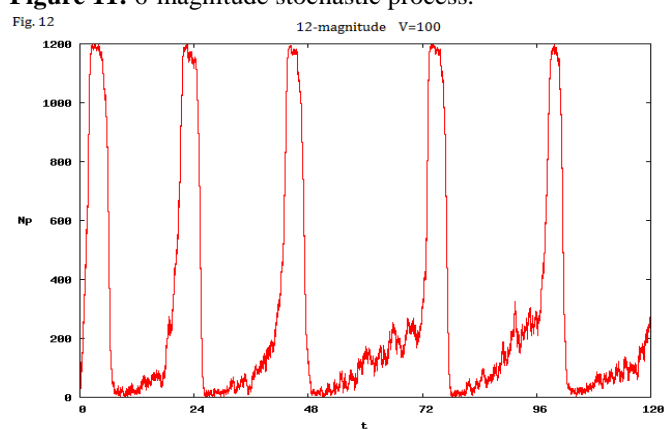
Figure 12: 12-magnitude stochastic process.
