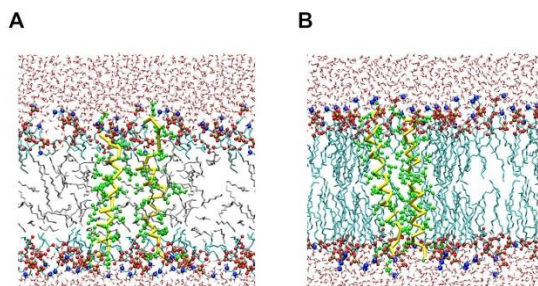
Figure 1: Representative snapshots of the dimerization PMF simulations. As examples, the systems for the poly-Leu peptides (KL22 w and KL22 y ) are shown. (A) The octane/diC 4 PC system (#2 of Table 1). In this example the interhelical distance r was held at 1.6 nm. Representation scheme: silver licorice, octane; spheres of middle size (ochre, red, and blue), diC 4 PC (phosphorus, oxygen, and nitrogen atoms, respectively); yellow trace, peptide backbone; green spheres, Leu side chains (SCs); thin licorice (silver and red), water atoms. Only lipid molecules located within a 2.0-nm-thick slice are shown. (B) The dioleoylphosphatidylcholine (DOPC) bilayer system (#1 of Table 1) with r was constrained at 1.1 nm. Representation scheme is similar to (A), but cyan licorice represents hydrocarbon chains of DOPC.
